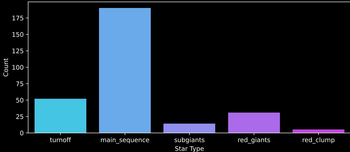
GALAH DR4 Field: [7013] Count plot of Star Type
