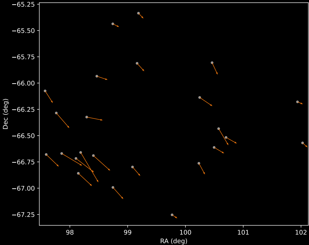
GALAH DR4 Cluster 2 Proper Motion Vectors (n=24)
