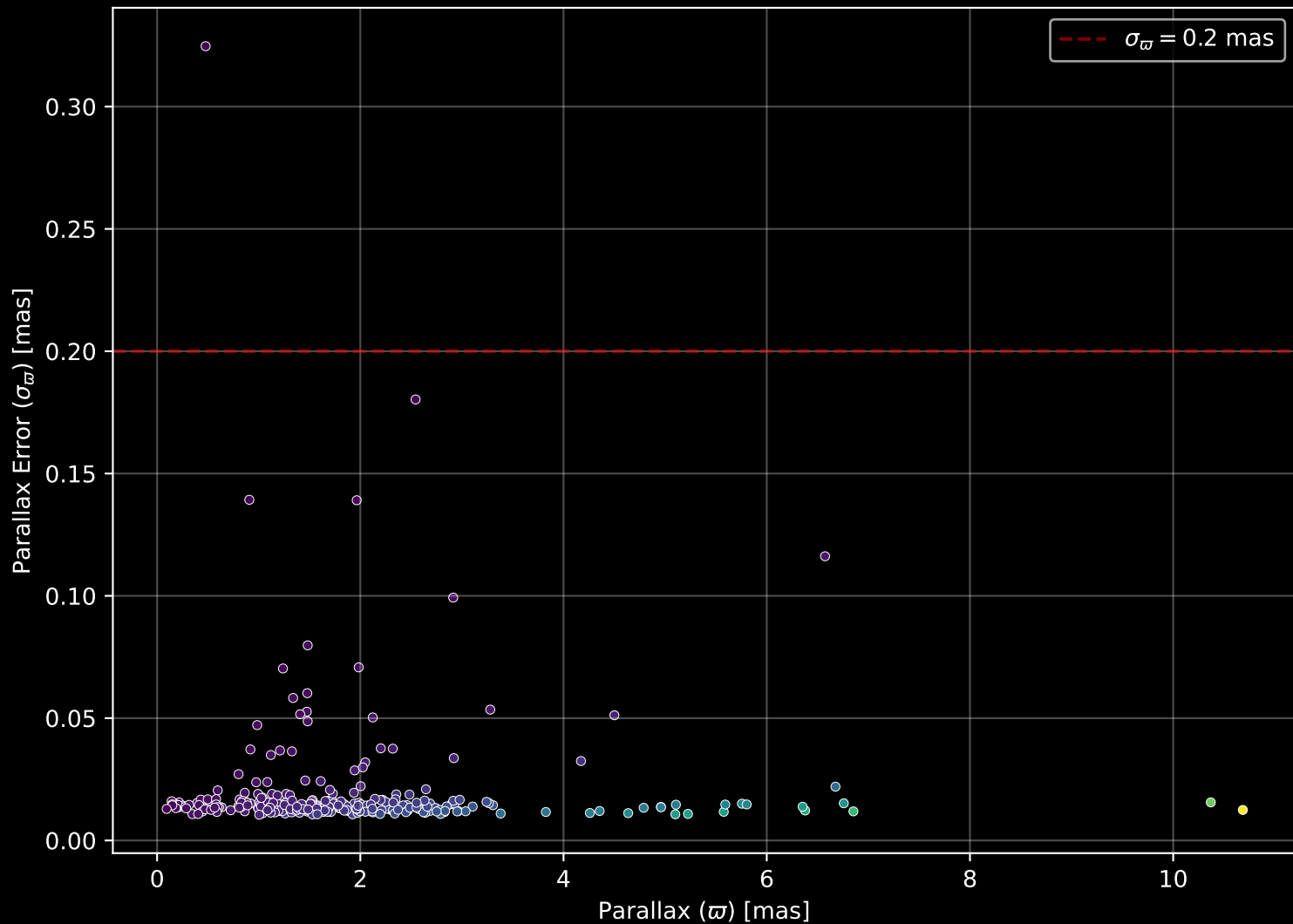
GALAH DR4 Field: [7013] Parallax Quality (n= 292)
