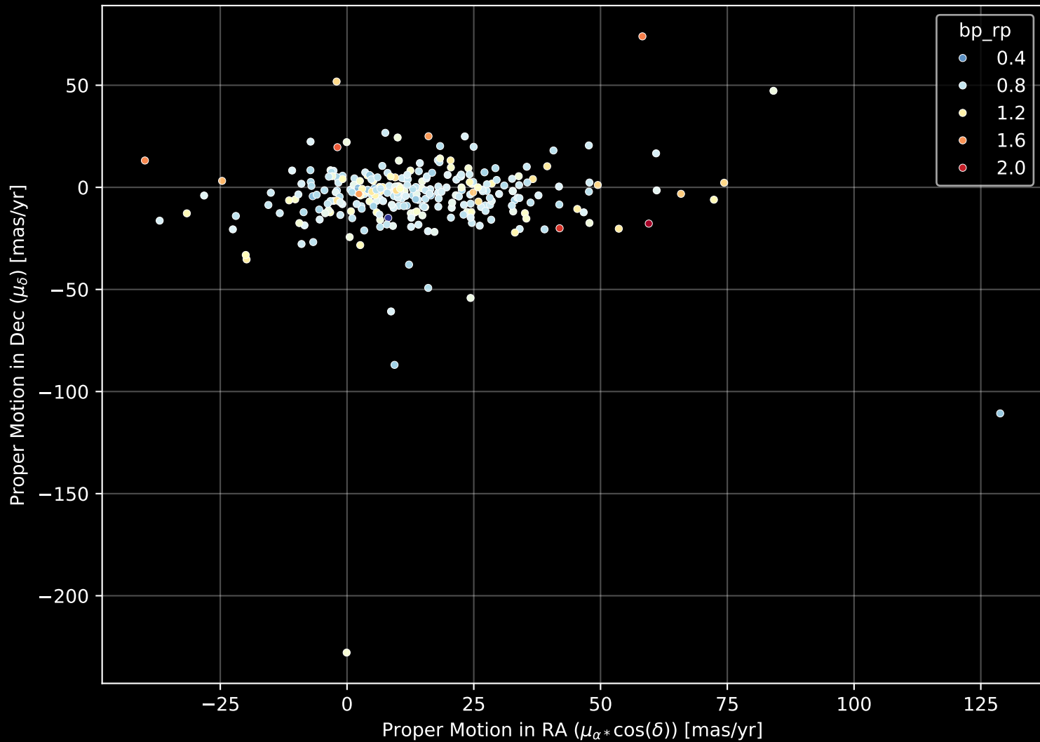
GALAH DR4 Field: [7013] Proper Motion Diagram (n= 292)
