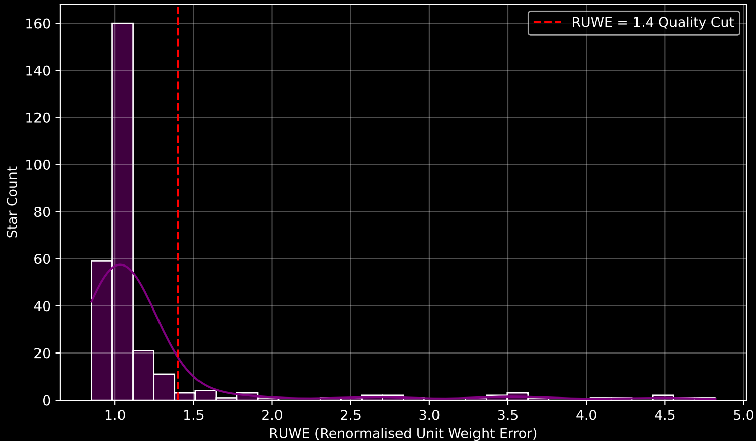
GALAH DR4 Field [7013] RUWE Distribution (n= 283)
