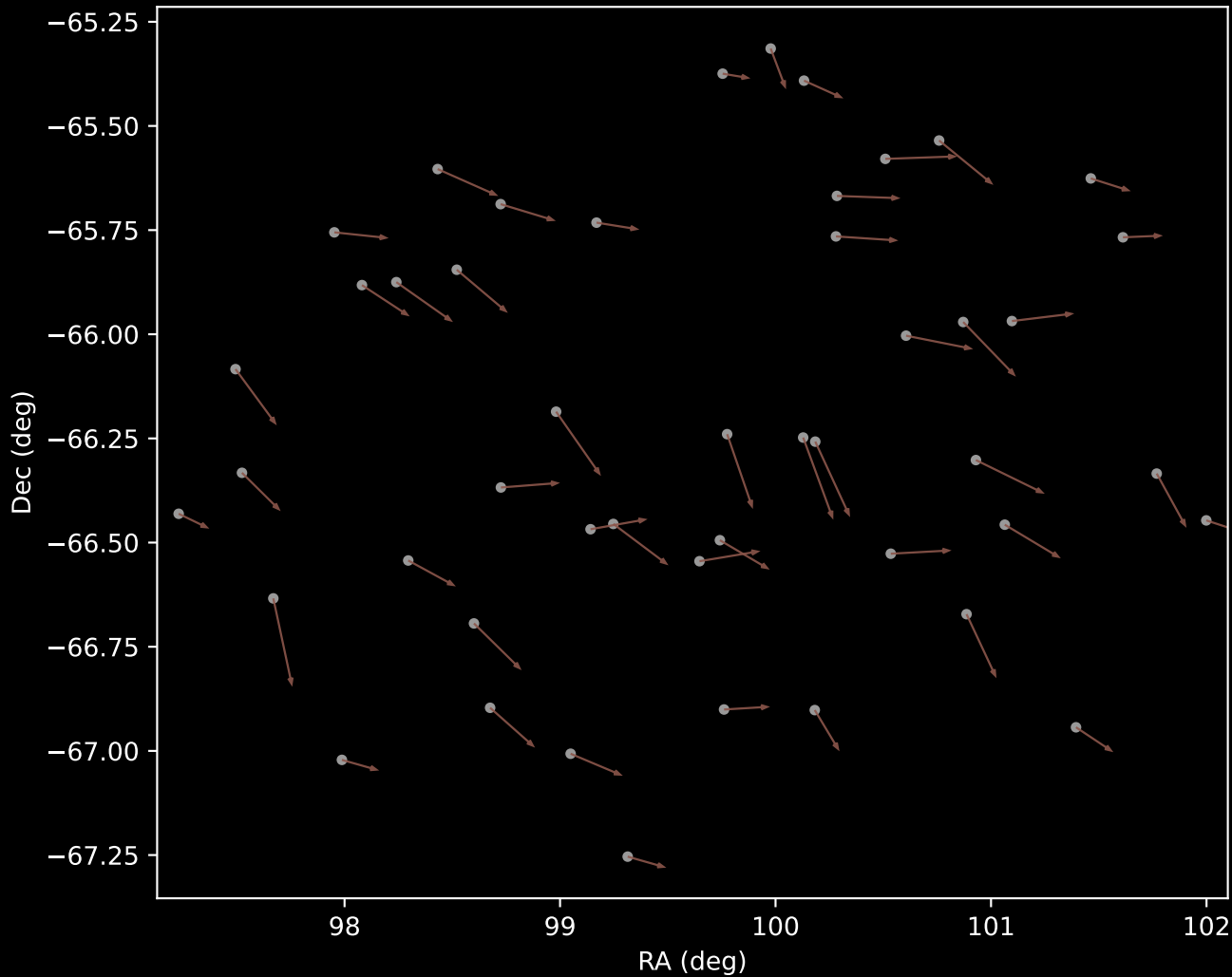
GALAH DR4 Cluster 10 Proper Motion Vectors (n=47)
